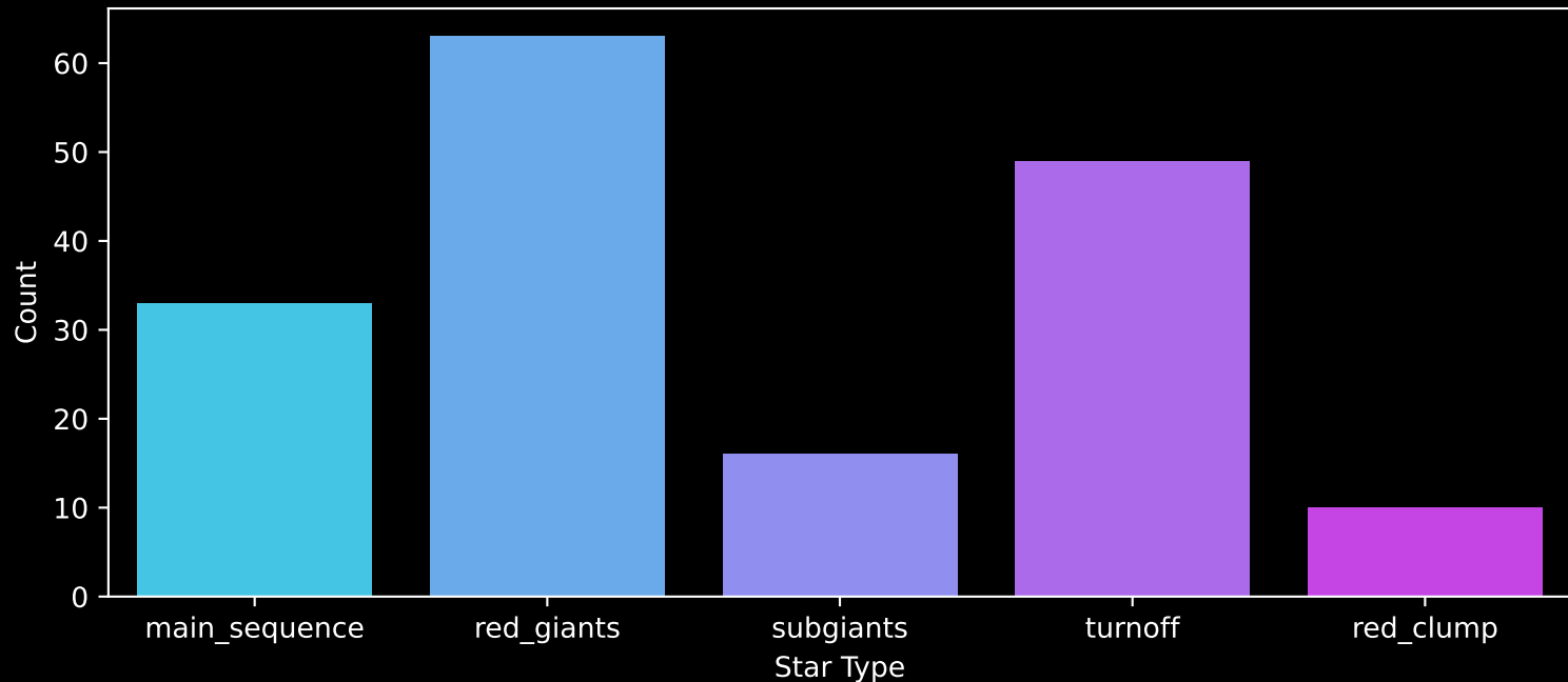
GALAH DR4 Field: [4120] Count plot of Star Type
