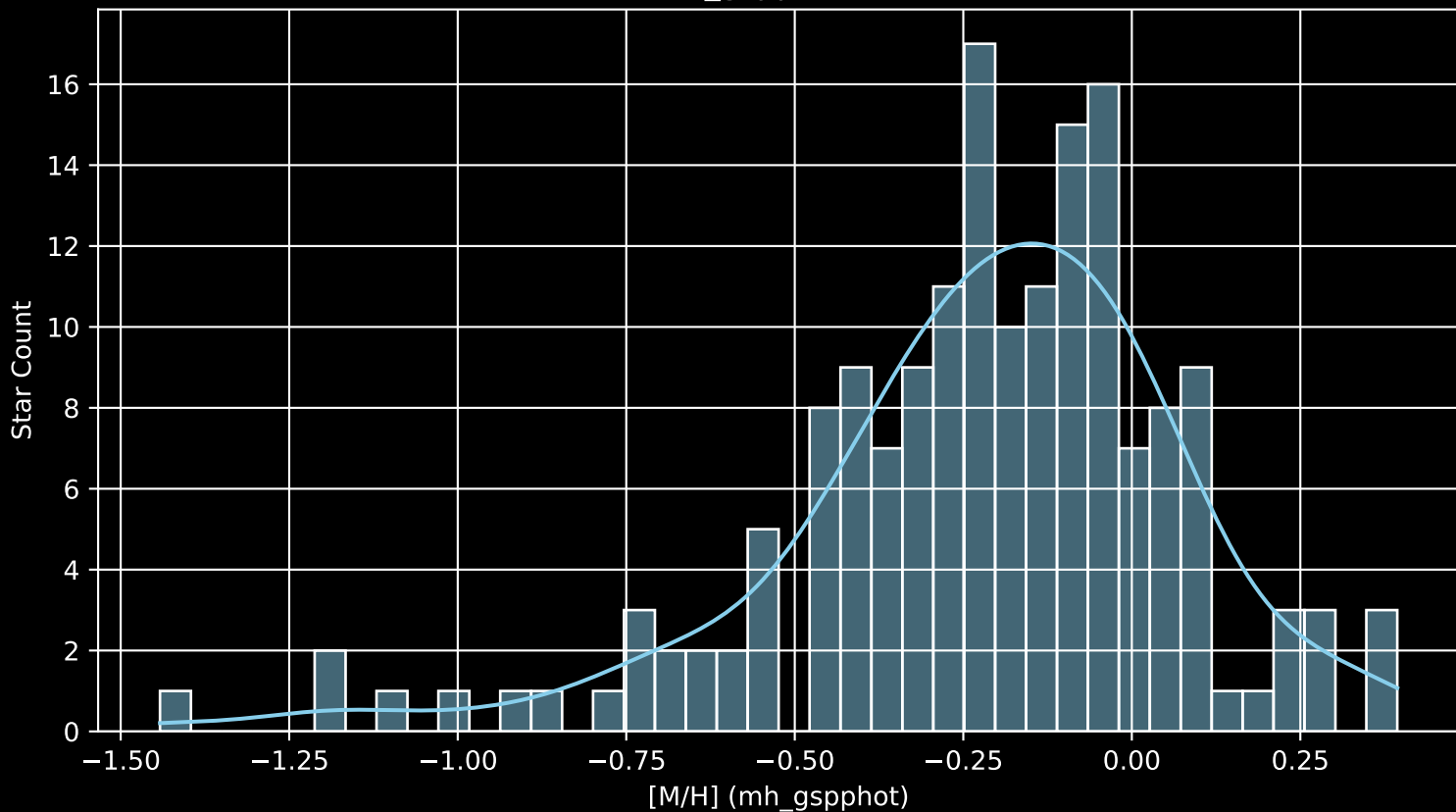
GALAH DR4 Field: [4120] [M/H] (mh_gspphot) (n= 170)
