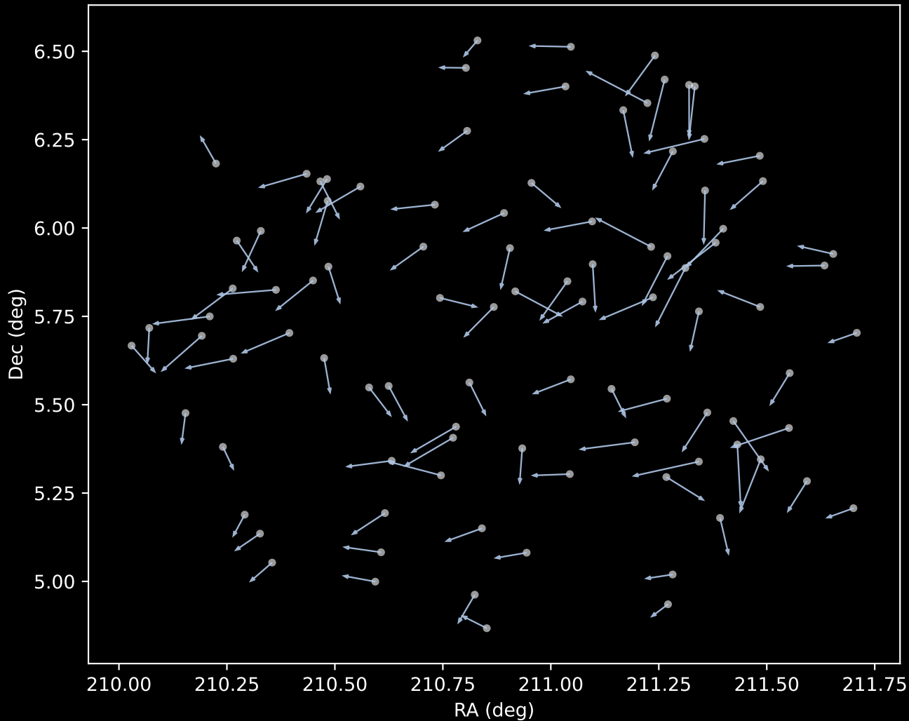
GALAH DR4 Cluster 1 Proper Motion Vectors (n=96)
