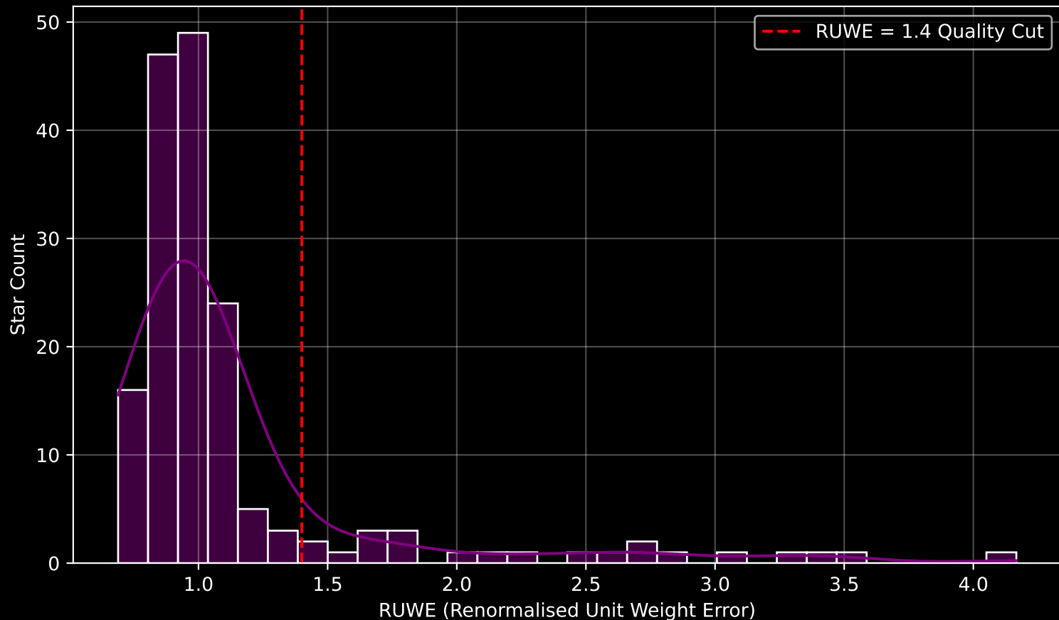
GALAH DR4 Field [4120] RUWE Distribution (n= 166)
